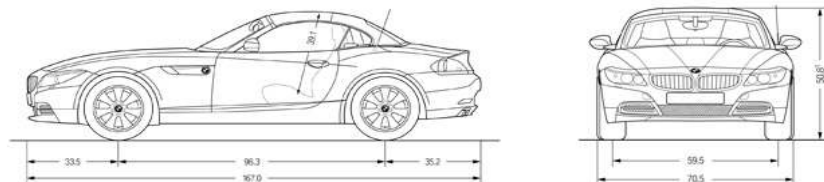
All dimensions in the technical drawings are given in inches. *Z4 sDrive35is: 50.6 inches.
